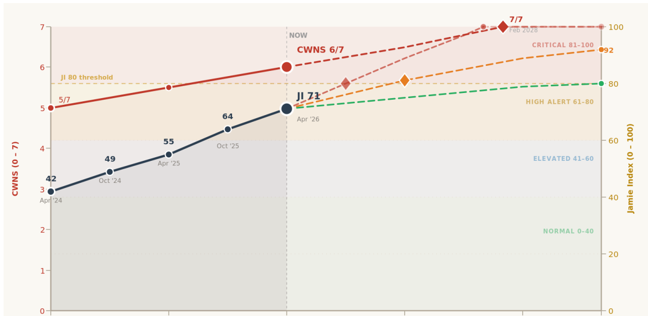
Figure 4: Jamie Index (gold, right axis 0–100) and Civil War Net Score (red, left axis 0–7) — April 2024 to December 2028 projected. Both instruments accelerate toward their respective outbreak thresholds (JI: 80, CWNS: 7/7) converging in Q4 2027–Q1 2028 — approximately 20–22 months from April 2026. Source: Jamie.Capital Research, Edition 16, March 2026.
